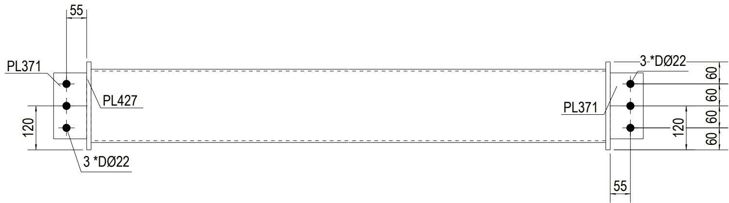
TOP VIEW
